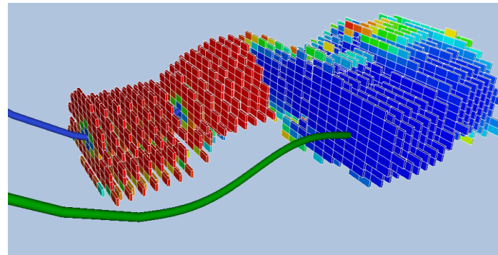
Example of interference on parent well from infill well
