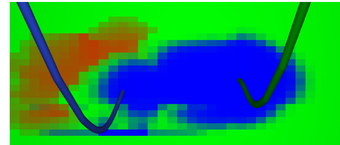
Ternary plot showing fracture to fracture interference
